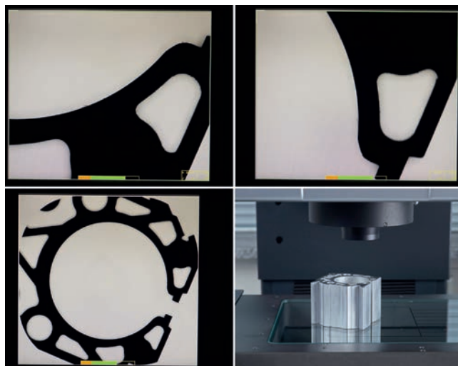
Figure 2. Tracing the workpiece edge with raster scanning using the image processing sensor (© Werth)
