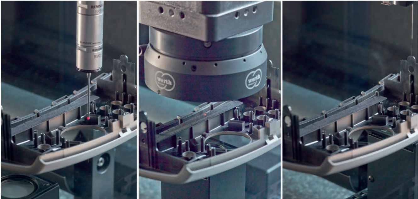
Figure 1. The datum features on a cover are defined using a conventional stylus system, then the flatness is measured with a laser distance sensor, and the flexible tab is measured with a fiber probe. (© Werth)
